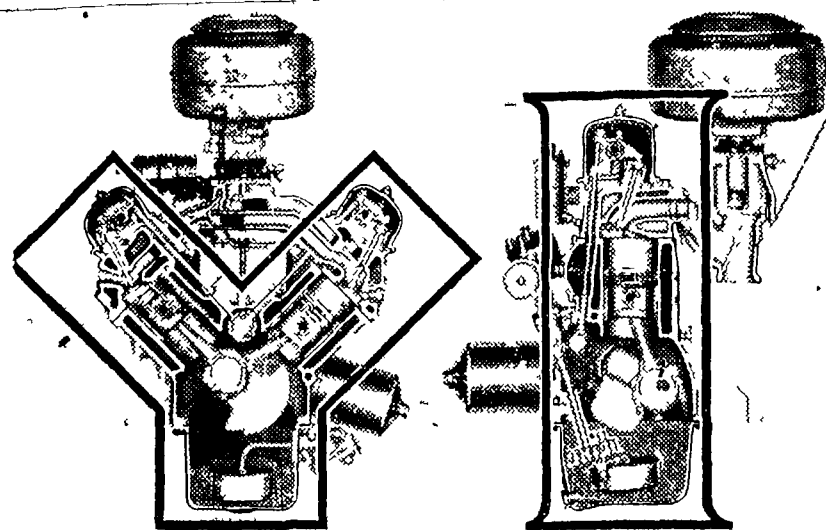
The new Y-block V-8
