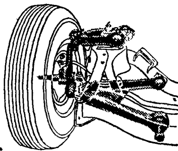
Ball-Joint Front Suspension
